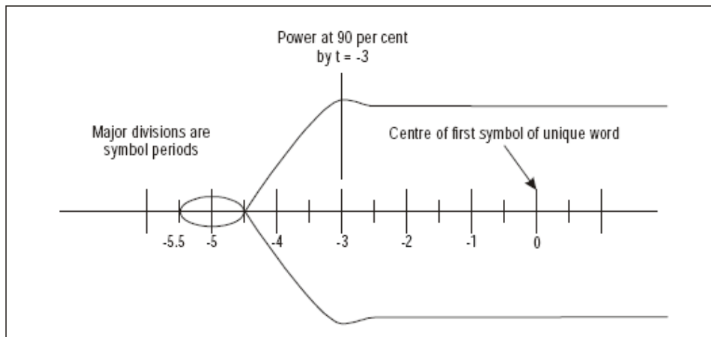
Figure 6-1. Transmitter power stabilization
