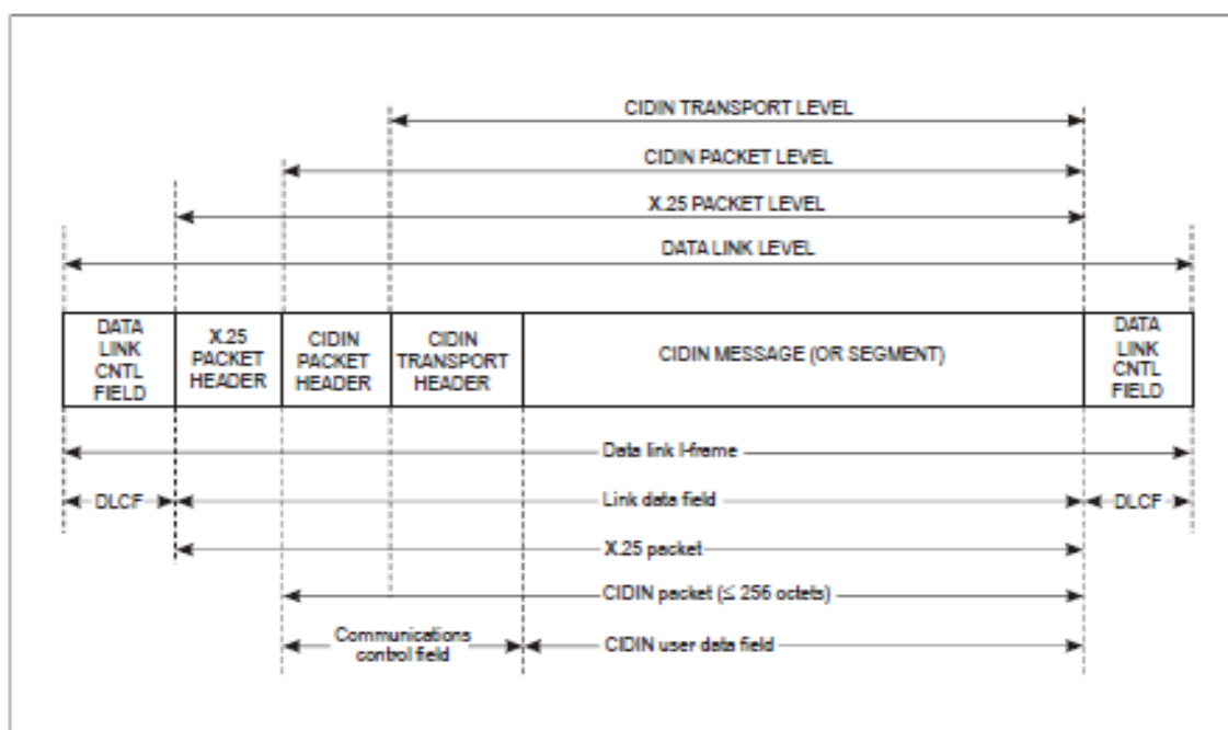
Figure 8-2. CIDIN terminology
