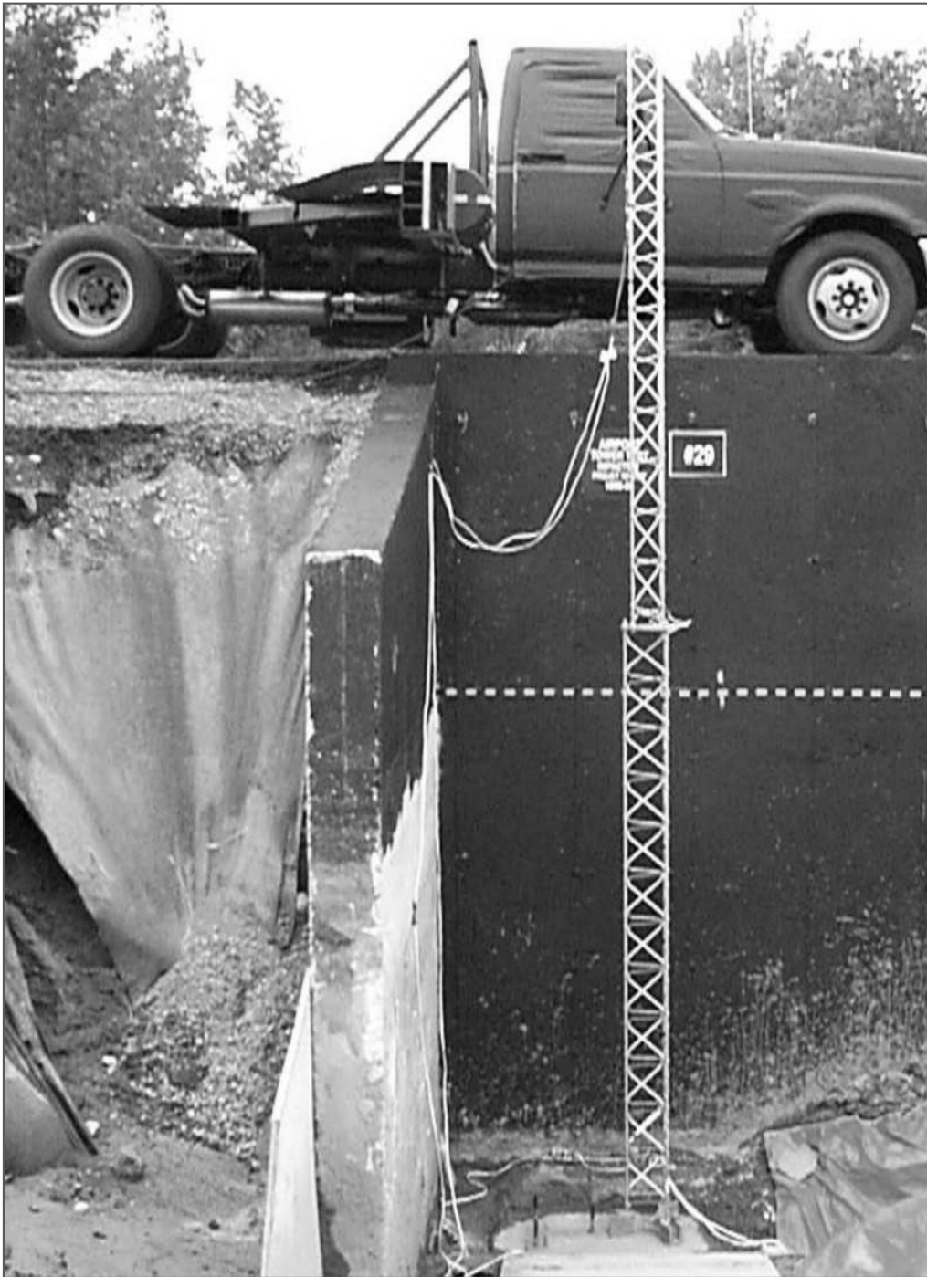
Figure 5-1. Example of general set-up for testing approach lighting towers With a vehicle-driven impacts.
