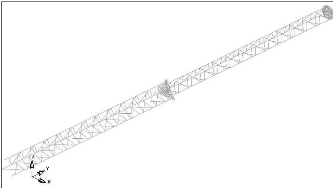
a) Approach lighting tower — fibreglass lattice structure
