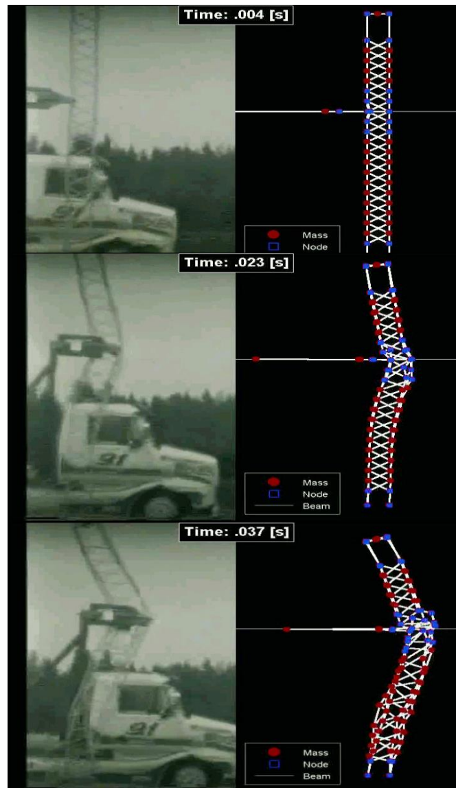
Figure 6-6. Comparison between actual deformation and that resulting from the hybrid analysis
