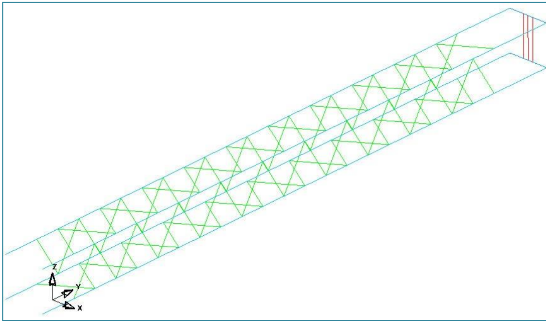
a) Approach lighting tower — fibreglass lattice structure
