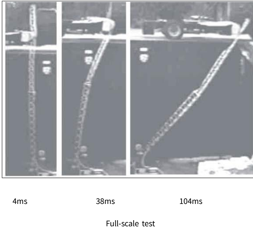
Figure 6-3. Impact events from finite element analysis (FEA) simulation and full-scale test — impact speed 140 km/h; impact on apex; top mass 5.44 kg; rigid impactor
