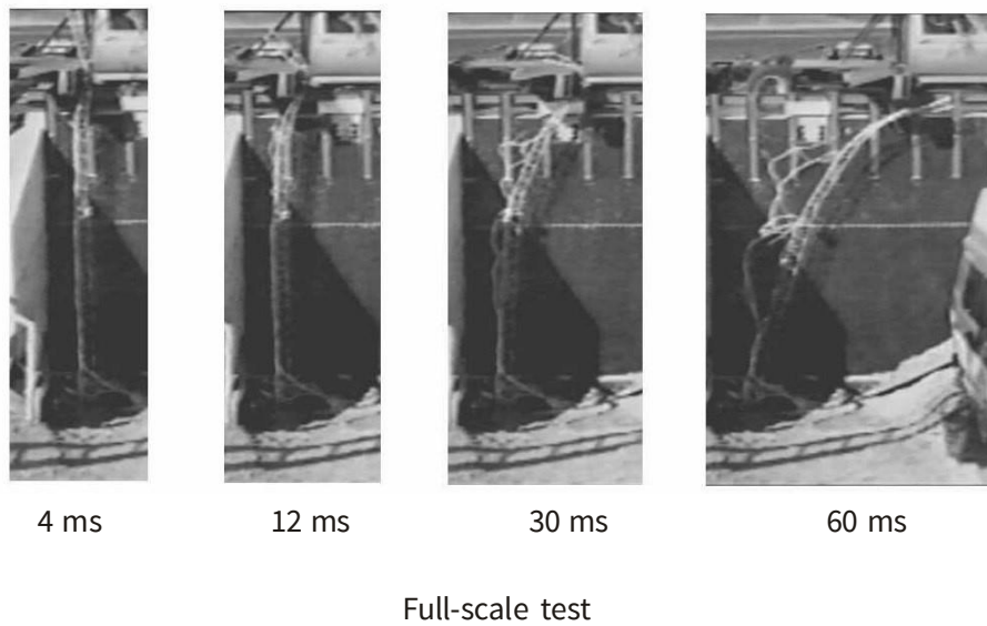
Figure 6-2. Impact events from finite element analysis (FEA) simulation and full-scale test — impact speed 140 km/h; impact on side; rigid impactor
